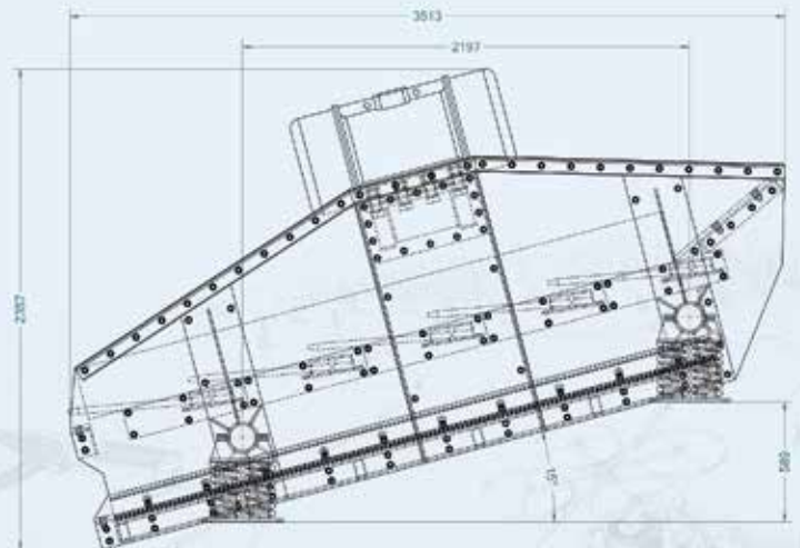
5' x 10' (1.5 m x 3.0 m) Rod Deck Screen, dimensions in mm.
