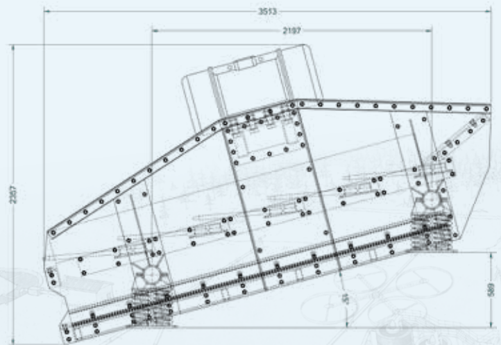
5' x 10' (1.5 m x 3.0 m) Rod Deck Screen, dimensions in mm.
